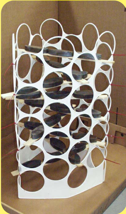
93lbs. of weight balanced on the Tomato Cage shows the strength and support.
